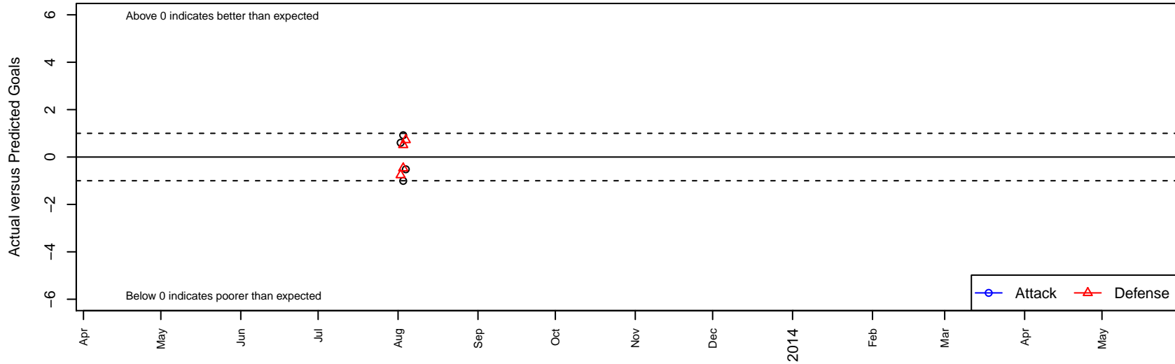
Rockets -Unk B97 Dots are actual minus expected GF (blue circles) and GA (red triangles). Blue line is smoothed change in attack strength. Red is smoothed change in defense strength.
